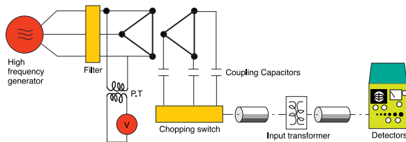
(CORONA TEST CIRCUIT)
